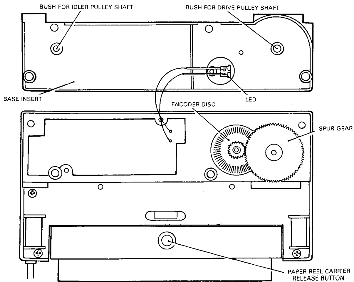
FIGURE 2 LOCATION OF COMPONENTS (2)
