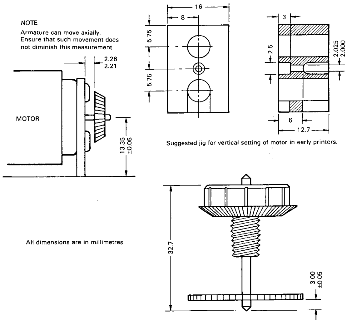
FIGURE 4 SETTING-UP DRIVE TRAIN
